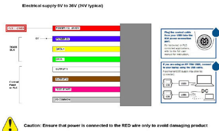
Figure 2 Wiring diagram for "P-version"
